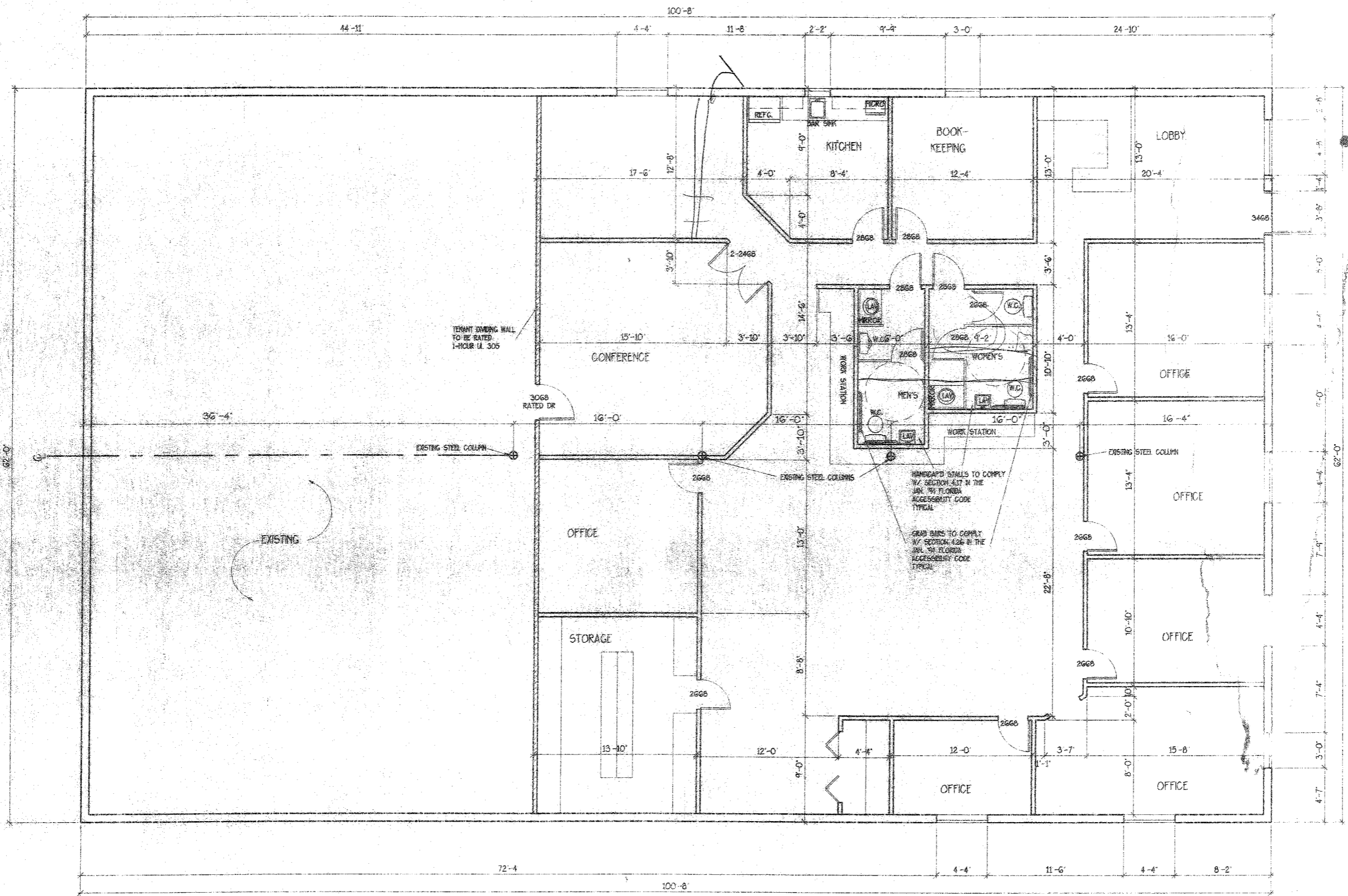
PROPOSED FLOOR PLAN SCALE: 1/4" = 1'-0"
